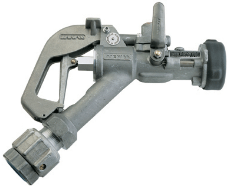
G2266-103: Automatic Nozzle w/ swivel
